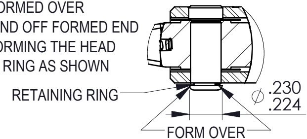
DETAIL B SCALE 1.5 : 1 DEFORM BEFORE CALIBRATION
